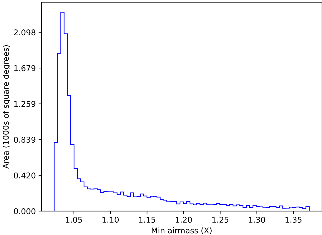
ddf_acor_sf15_lsf30_lsr50_v3.4_10yrs WFD g band: Min airmass
