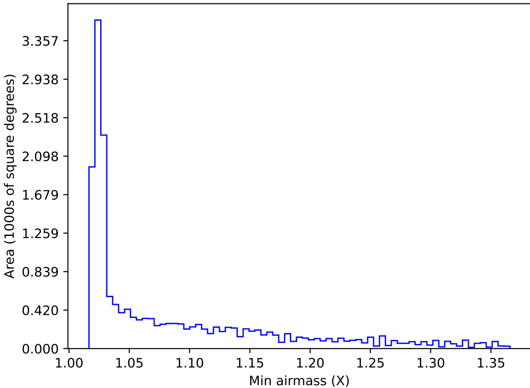
ddf_acor_sf15_lsf30_lsr50_v3.4_10yrs WFD all bands: Min airmass
