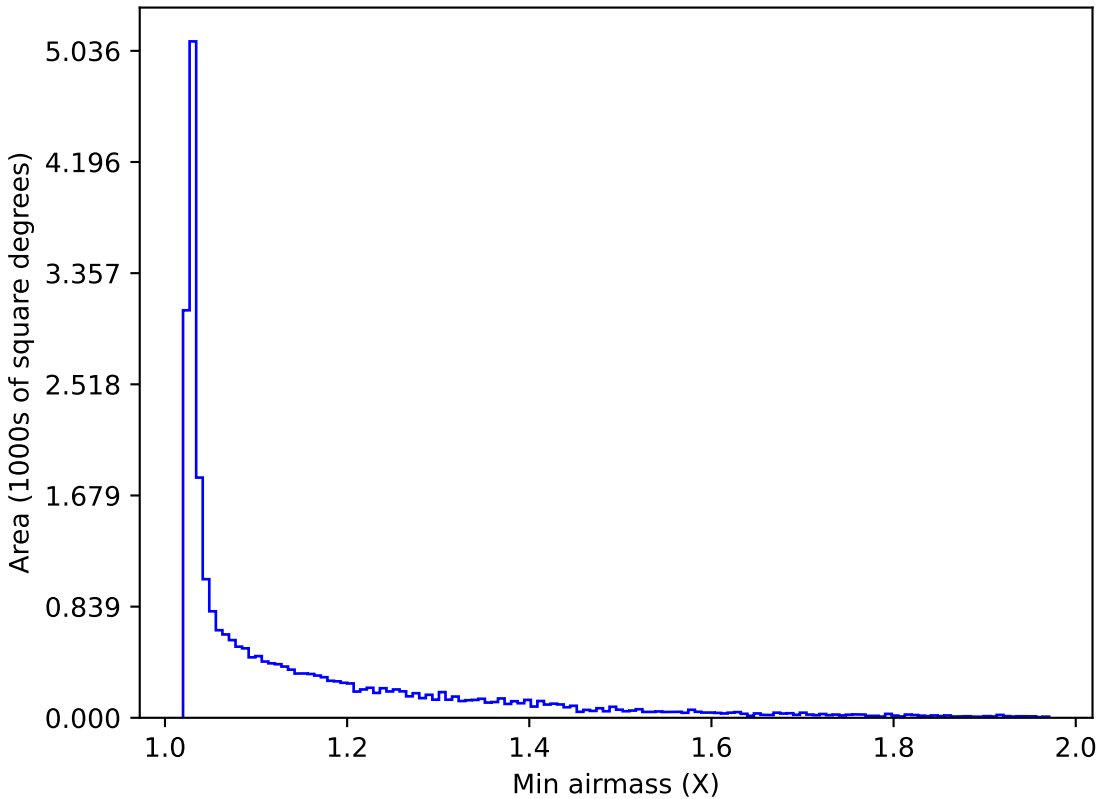
ddf_acor_sf15_lsf30_lsr50_v3.4_10yrs All sky z band: Min airmass
