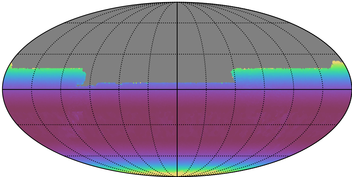
ddf_acor_sf15_lsf30_lsr50_v3.4_10yrs All sky y band: Min airmass
