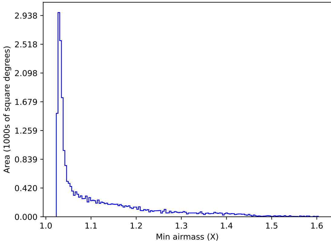
ddf_acor_sf15_lsf30_lsr50_v3.4_10yrs All sky y band: Min airmass
