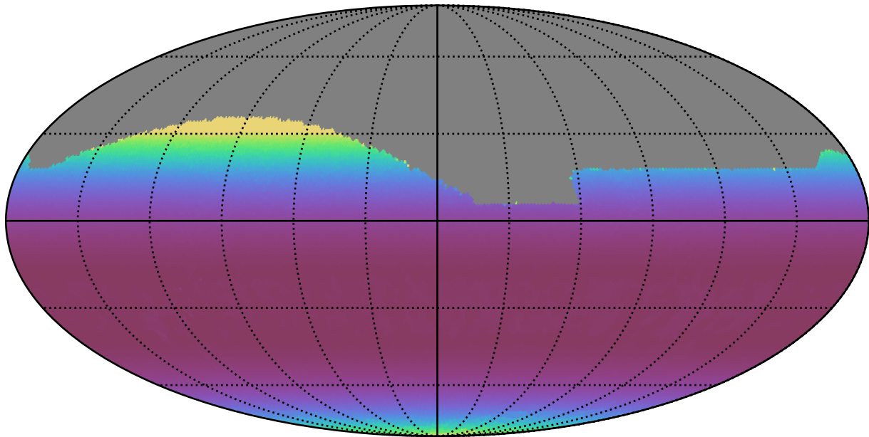
ddf_acor_sf15_lsf30_lsr50_v3.4_10yrs All sky r band: Min airmass
