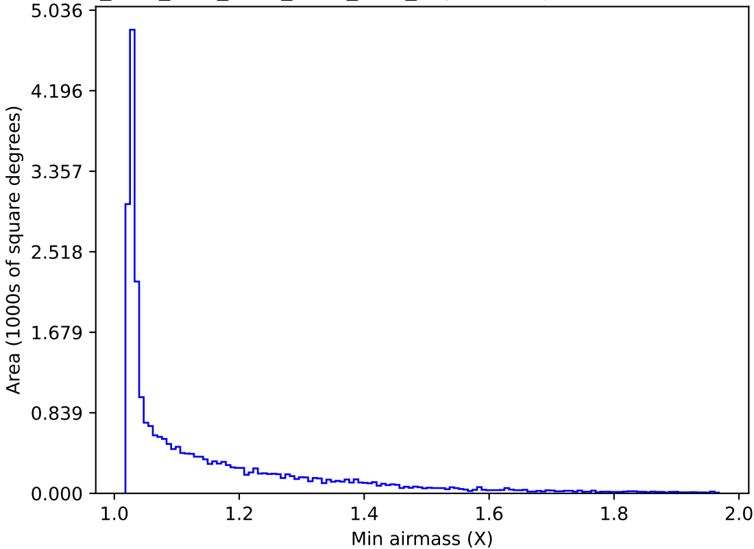
ddf_acor_sf15_lsf30_lsr50_v3.4_10yrs All sky r band: Min airmass
