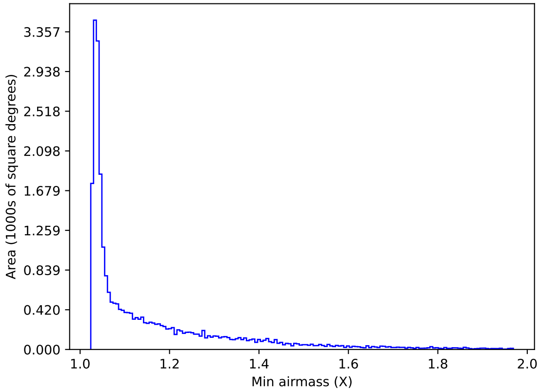
ddf_acor_sf15_lsf30_lsr50_v3.4_10yrs All sky g band: Min airmass
