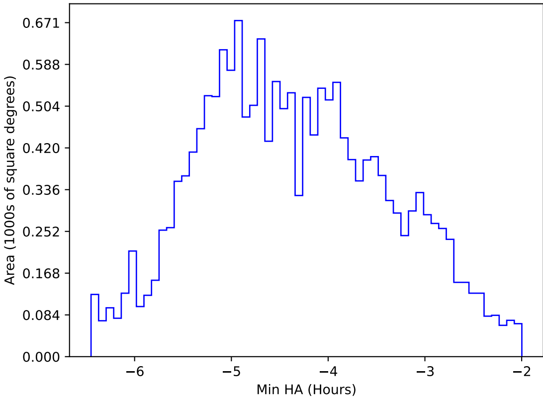
ddf_acor_sf15_lsf30_lsr50_v3.4_10yrs WFD i band: Min HA
