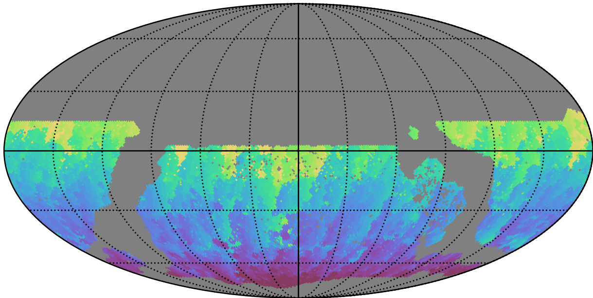
ddf_acor_sf15_lsf30_lsr50_v3.4_10yrs WFD g band: Min HA
