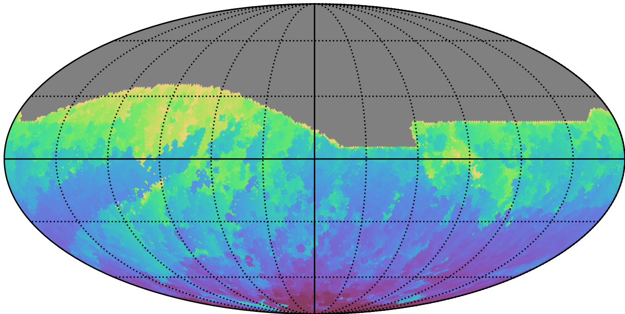
ddf_acor_sf15_lsf30_lsr50_v3.4_10yrs All sky z band: Min HA
