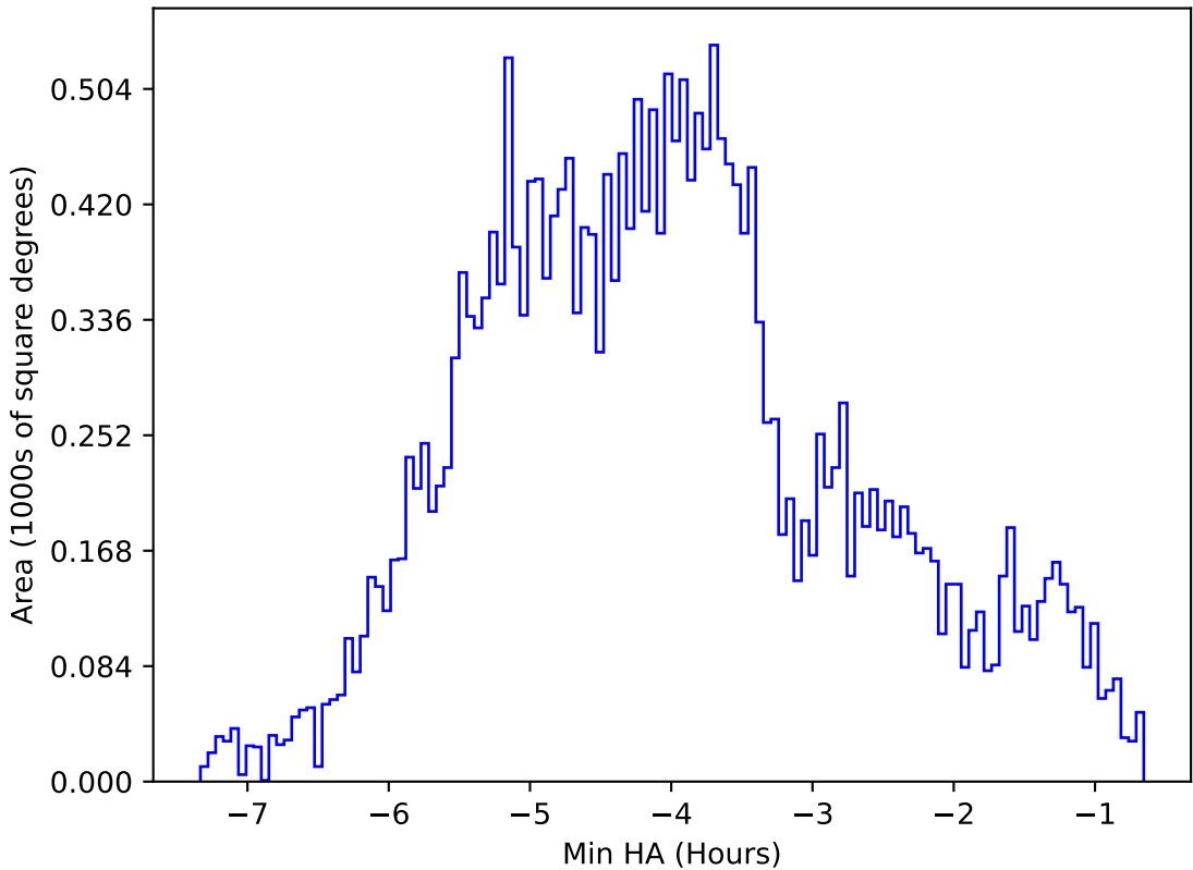
ddf_acor_sf15_lsf30_lsr50_v3.4_10yrs All sky z band: Min HA
