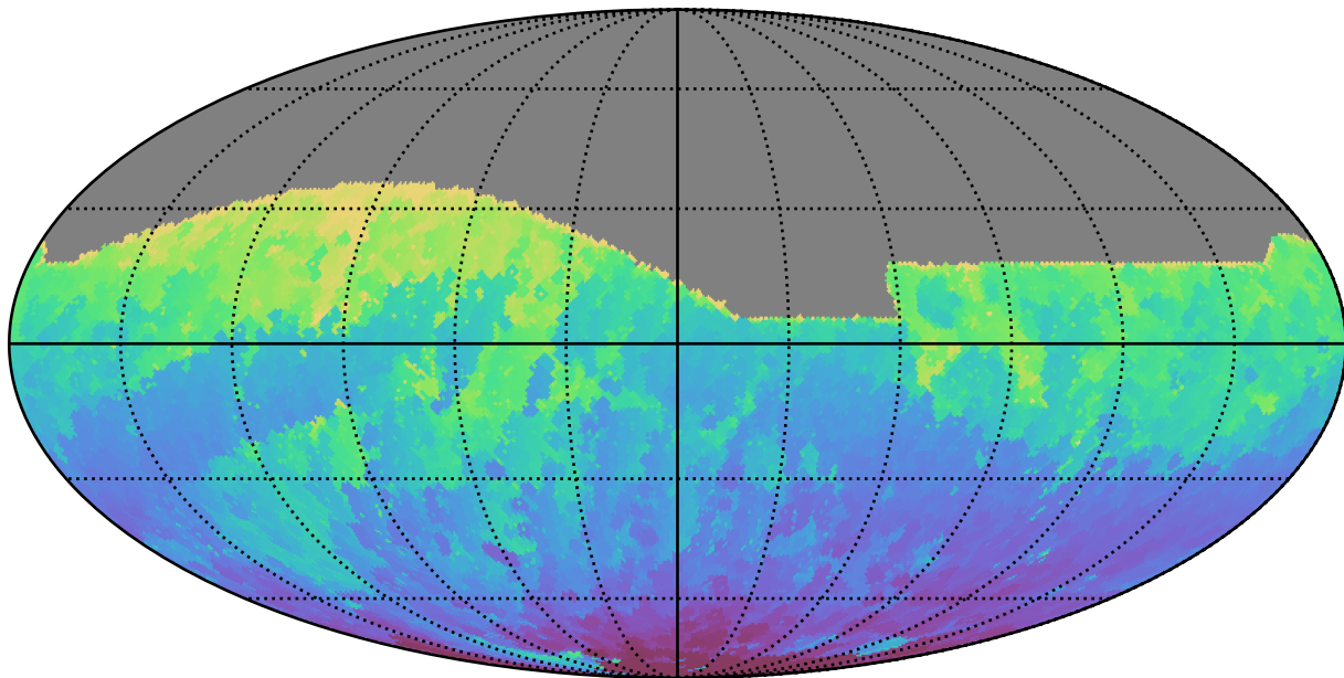
ddf_acor_sf15_lsf30_lsr50_v3.4_10yrs All sky i band: Min HA
