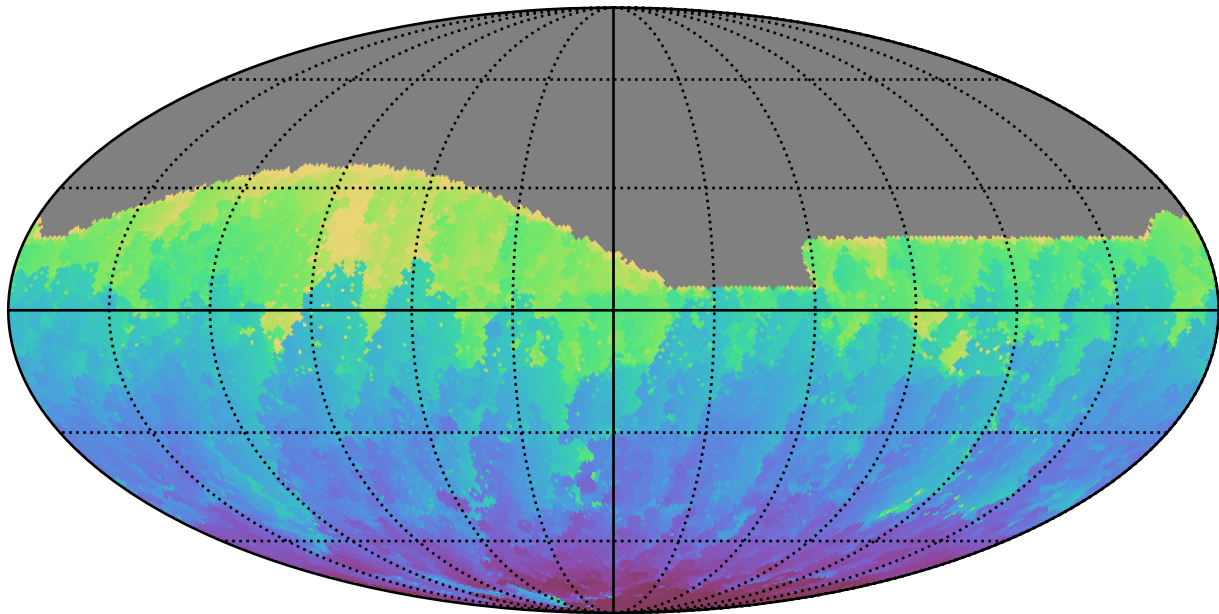
ddf_acor_sf15_lsf30_lsr50_v3.4_10yrs All sky g band: Min HA
