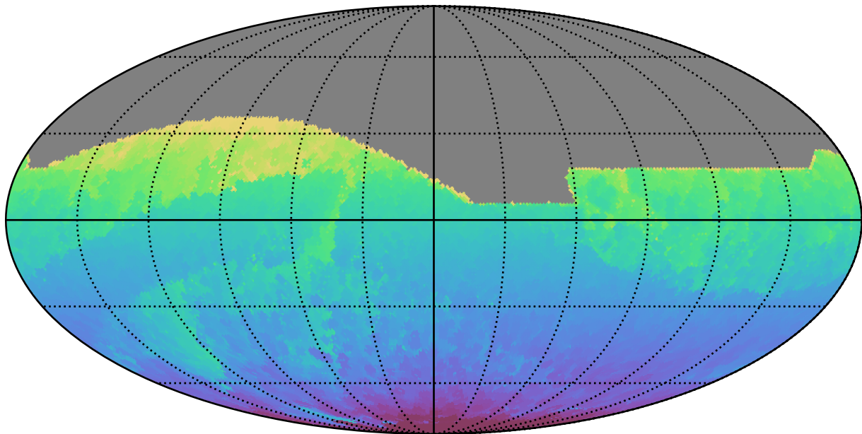
ddf_acor_sf15_lsf30_lsr50_v3.4_10yrs All sky all bands: Min HA
