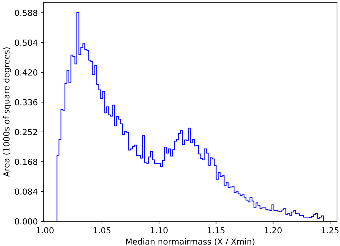
ddf_acor_sf15_lsf30_lsr50_v3.4_10yrs All sky u band: Median normairmass
