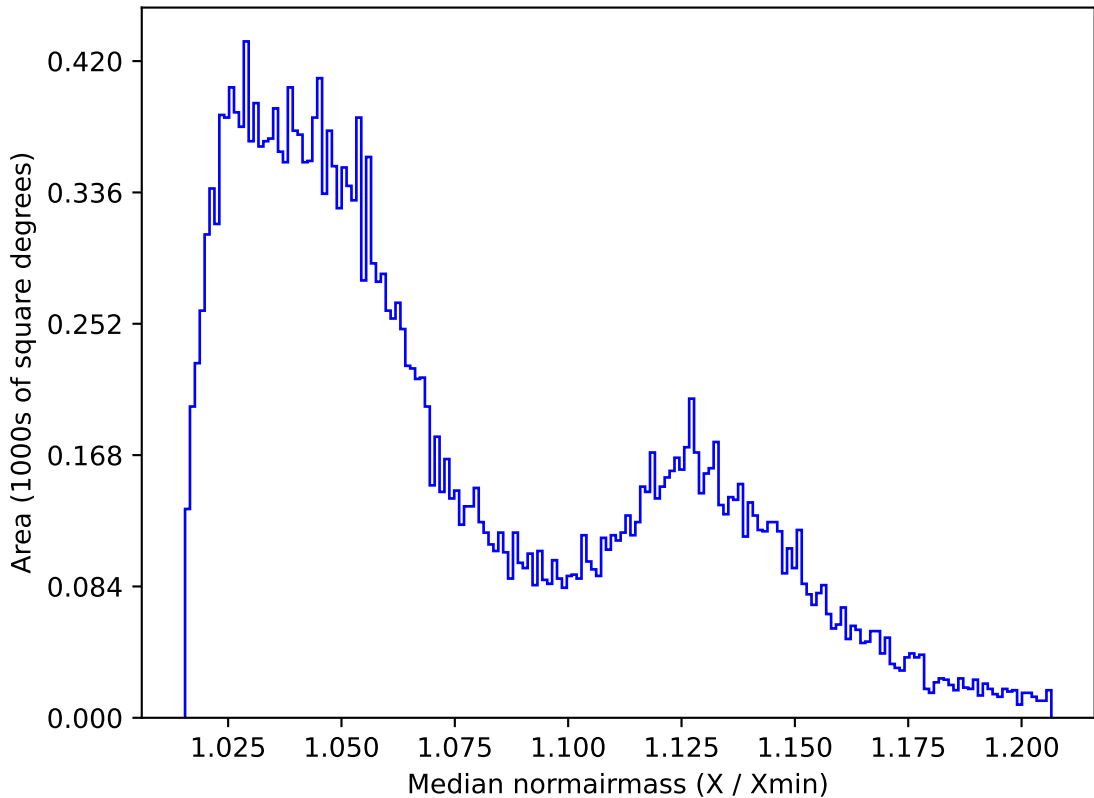
ddf_acor_sf15_lsf30_lsr50_v3.4_10yrs All sky r band: Median normairmass
