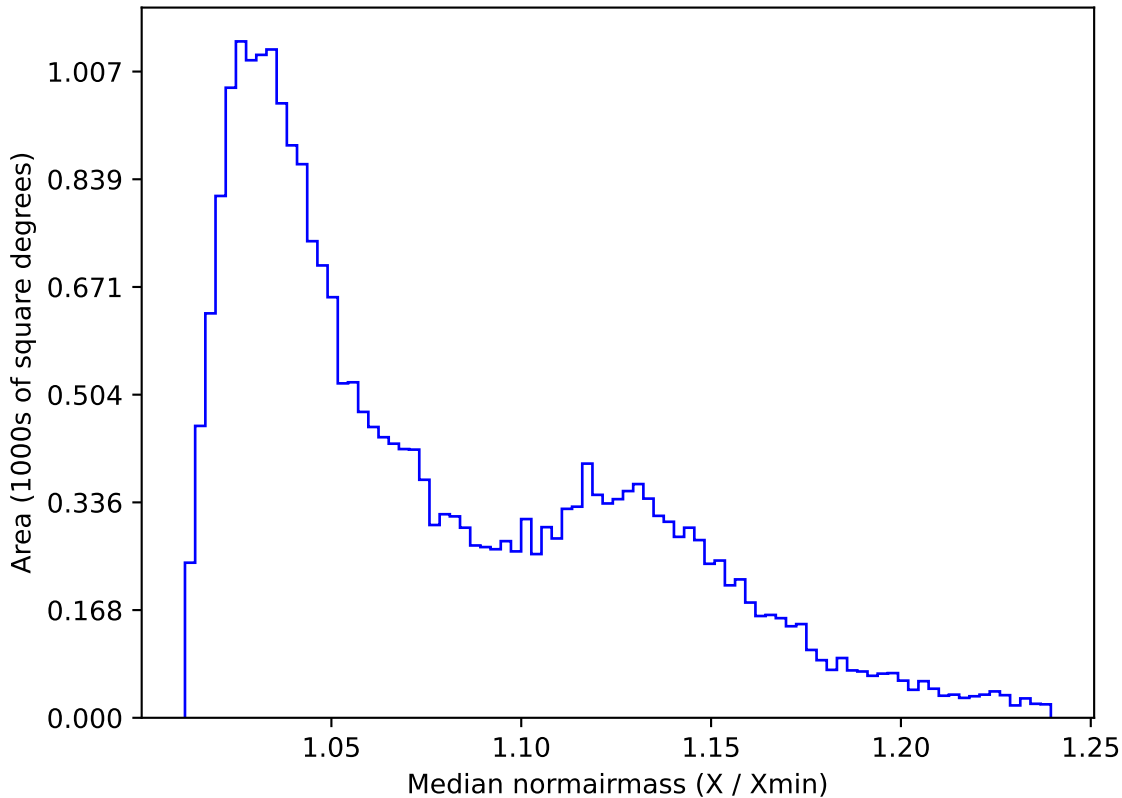
ddf_acor_sf15_ls30_lsr50_v3.4_10yrs All sky g band: Median normairmass
