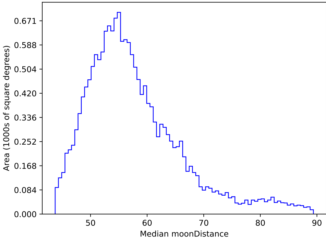
ddf_acor_sf15_lsf30_lsr50_v3.4_10yrs WFD y band: Median moonDistance
