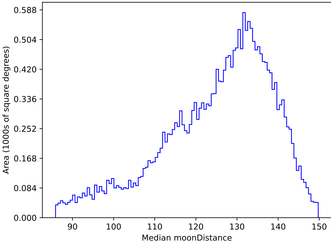
ddf_acor_sf15_lsf30_lsr50_v3.4_10yrs All sky u band: Median moonDistance
