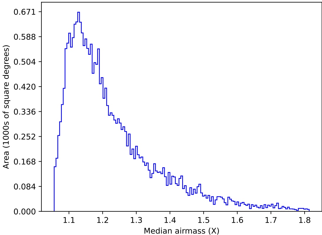
ddf_acor_sf15_lsf30_lsr50_v3.4_10yrs Yr 1 u band: Median airmass
