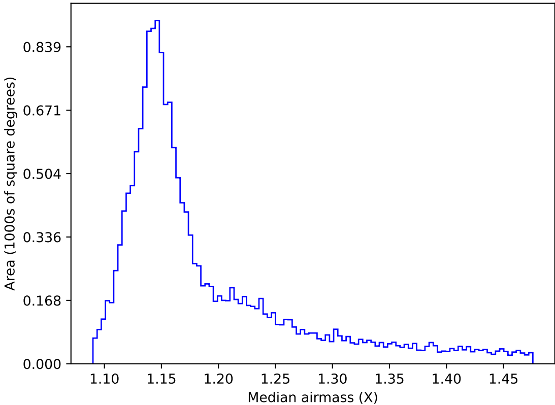
ddf_acor_sf15_lsf30_lsr50_v3.4_10yrs WFD y band: Median airmass
