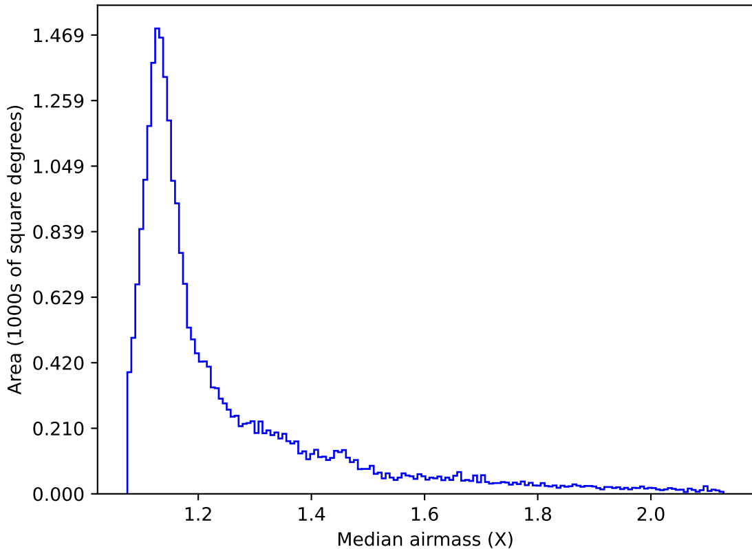
ddf_acor_sf15_lsf30_lsr50_v3.4_10yrs All sky g band: Median airmass
