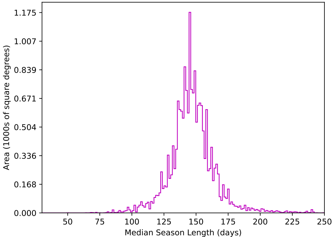
ddf_acor_sf15_lsf30_lsr50_v3.4_10yrs WFD z band: Median Season Length
