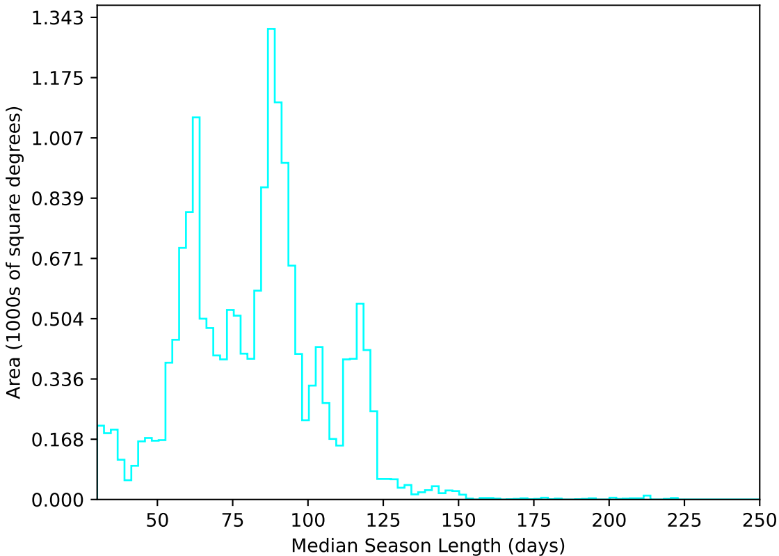
ddf_acor_sf15_lsf30_lsr50_v3.4_10yrs WFD u band: Median Season Length
