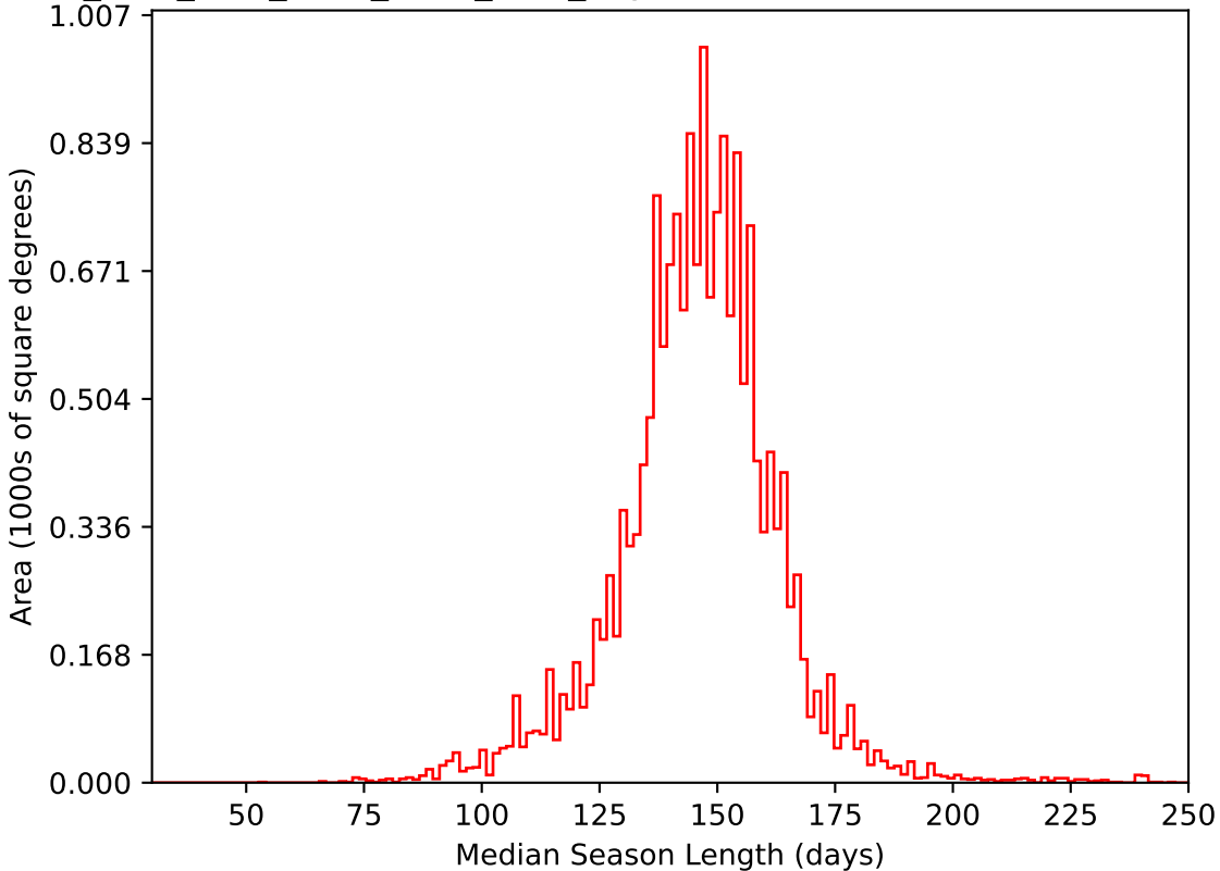
ddf_acor_sf15_lsf30_lsr50_v3.4_10yrs WFD i band: Median Season Length
