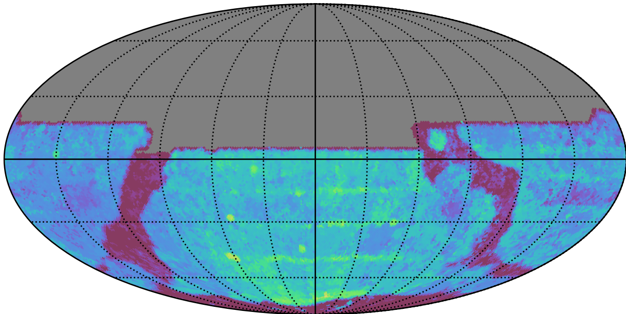
ddf_acor_sf15_lsf30_lsr50_v3.4_10yrs All sky y band: Median Season Length
