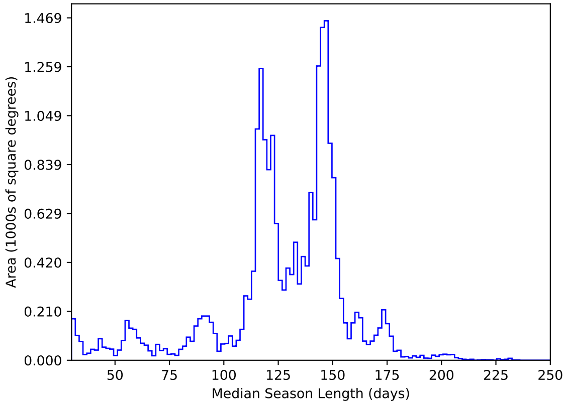
ddf_acor_sf15_lsf30_lsr50_v3.4_10yrs All sky y band: Median Season Length
