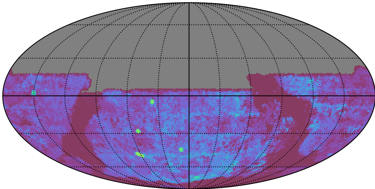
ddf_acor_sf15_lsf30_lsr50_v3.4_10yrs All sky u band: Median Season Length
