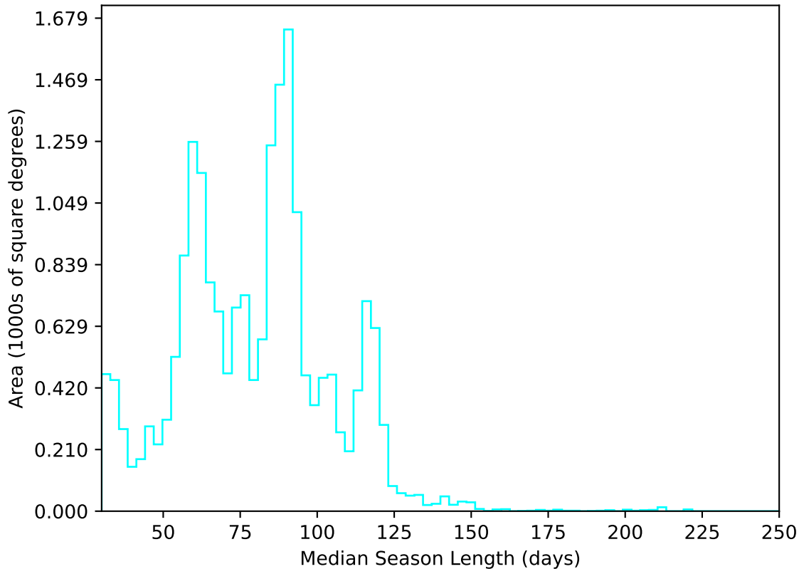
ddf_acor_sf15_lsf30_lsr50_v3.4_10yrs All sky u band: Median Season Length
