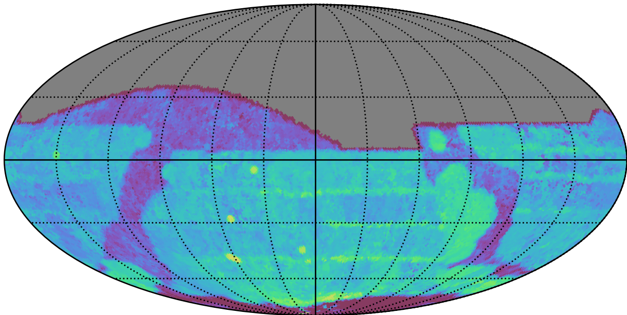
ddf_acor_sf15_lsf30_lsr50_v3.4_10yrs All sky r band: Median Season Length
