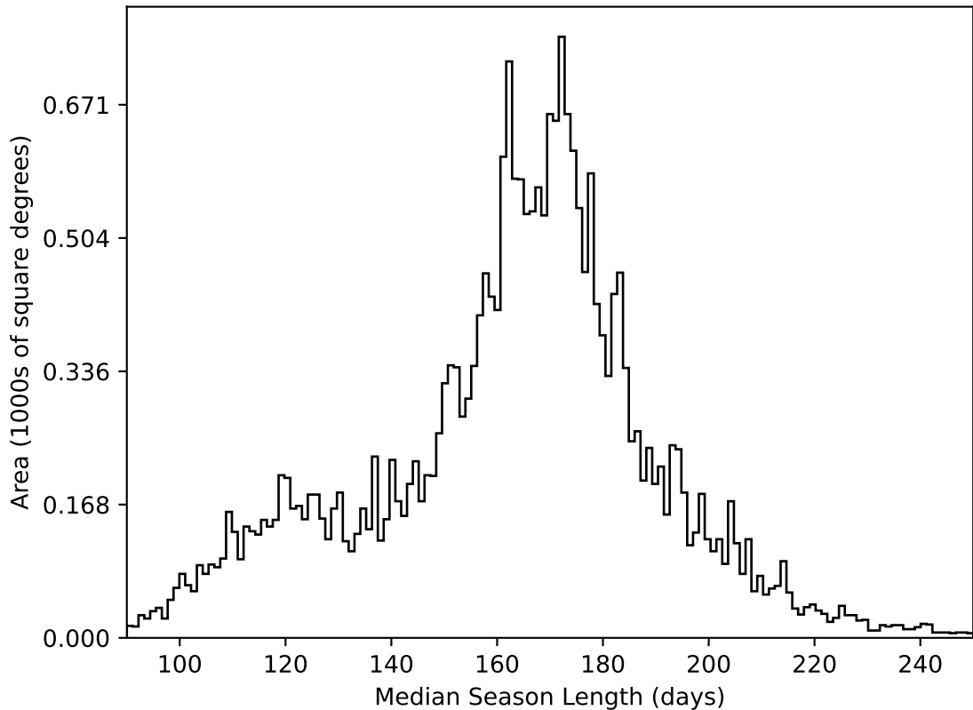
ddf_acor_sf15_lsf30_lsr50_v3.4_10yrs All sky all bands: Median Season Length
