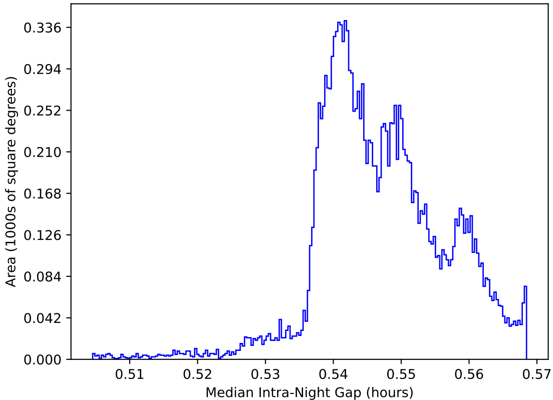
ddf_acor_sf15_ls30_lsr50_v3.4_10yrs WFD: Median Intra-Night Gap
