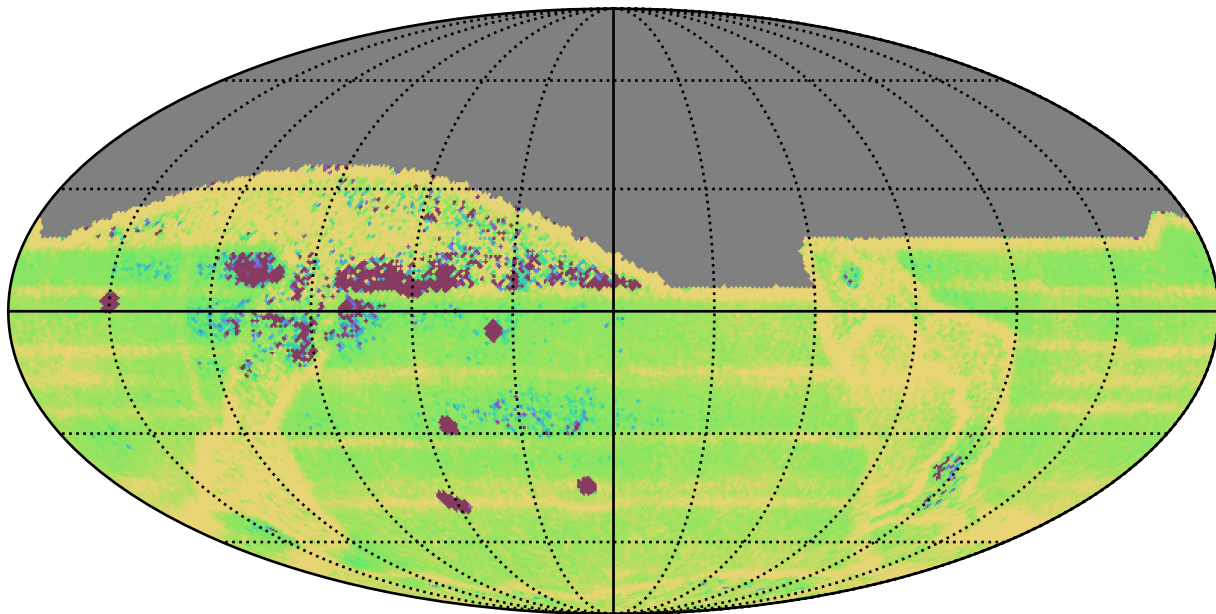
ddf_acor_sf15_lsf30_lsr50_v3.4_10yrs All sky: Median Intra-Night Gap
