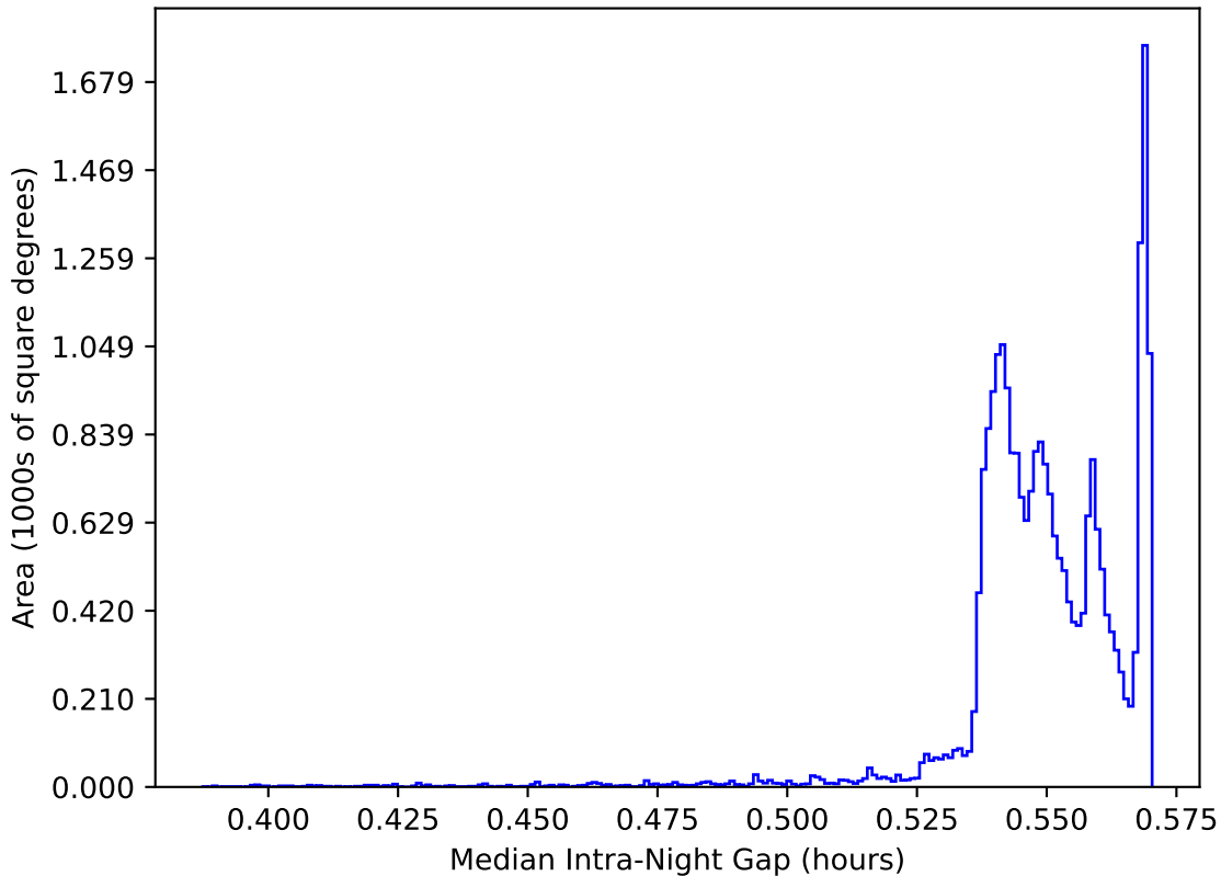
ddf_acor_sf15_lsf30_lsr50_v3.4_10yrs All sky: Median Intra-Night Gap
