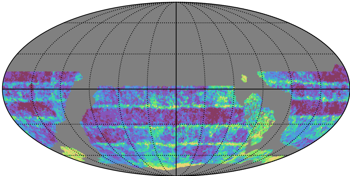
ddf_acor_sf15_lsf30_lsr50_v3.4_10yrs WFD r band: Median Inter-Night Gap
