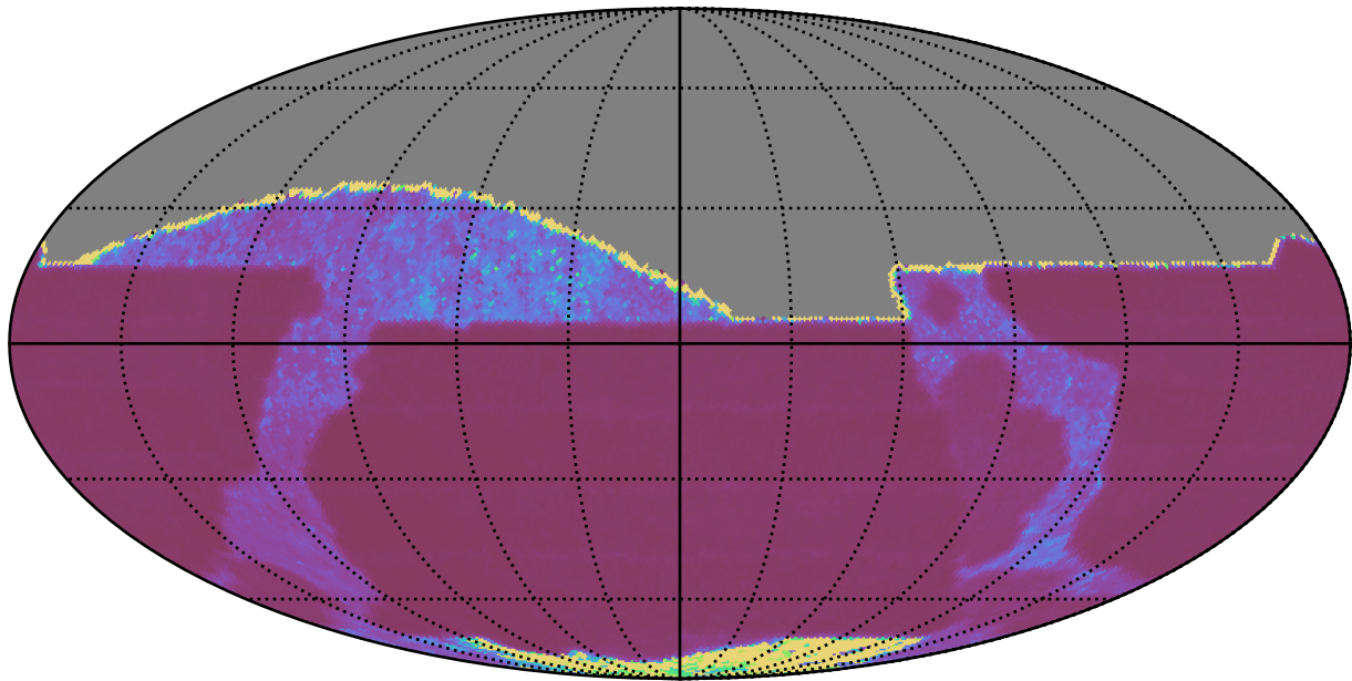
ddf_acor_sf15_lsf30_lsr50_v3.4_10yrs All sky z band: Median Inter-Night Gap
