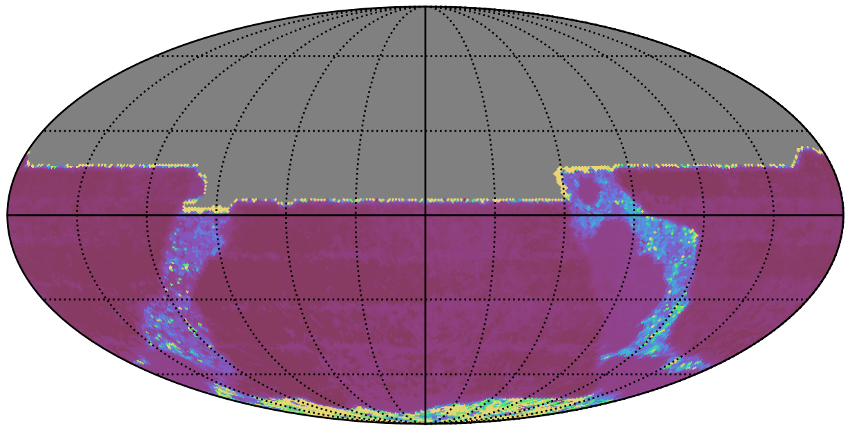
ddf_acor_sf15_lsf30_lsr50_v3.4_10yrs All sky y band: Median Inter-Night Gap
