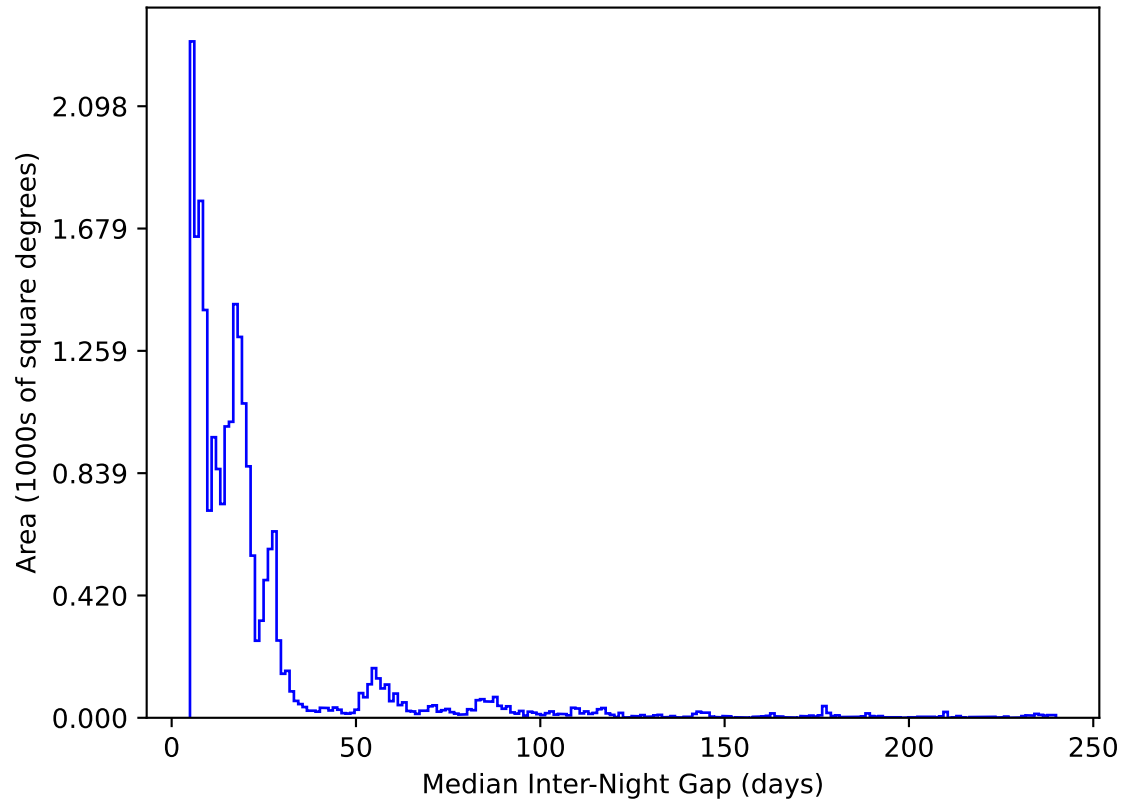
ddf_acor_sf15_lsf30_lsr50_v3.4_10yrs All sky y band: Median Inter-Night Gap
