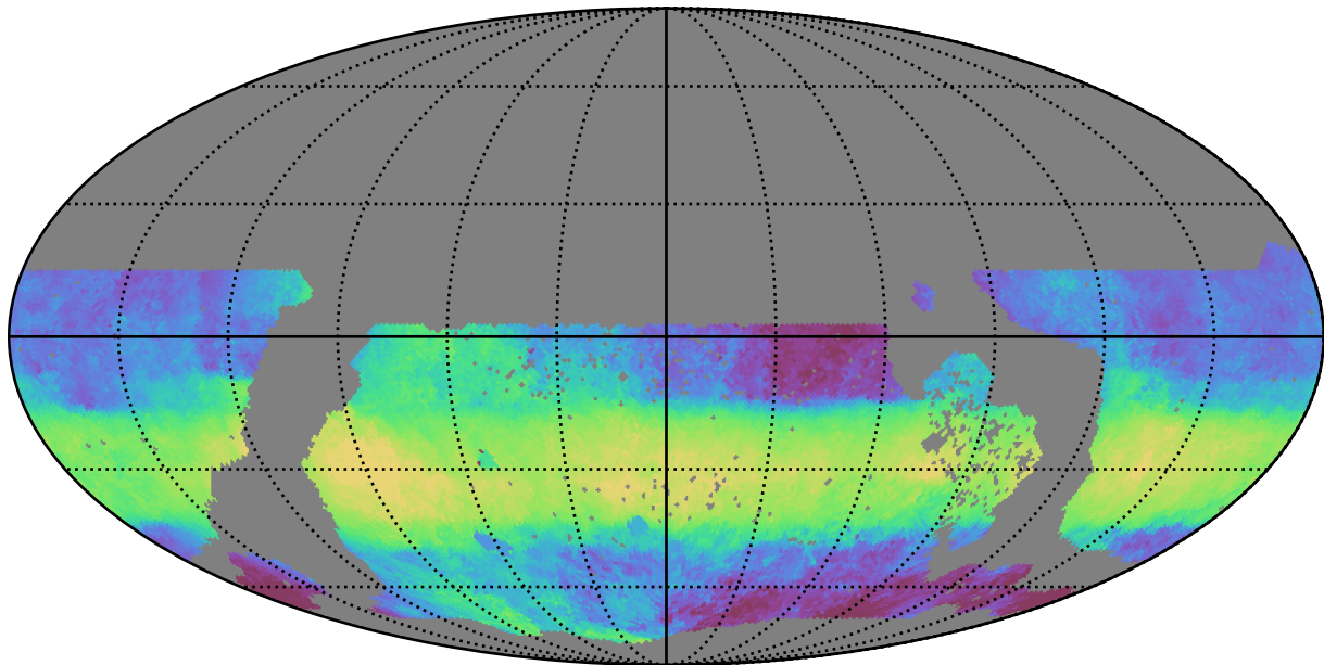
ddf_acor_sf15_lsf30_lsr50_v3.4_10yrs WFD z band: Median HA
