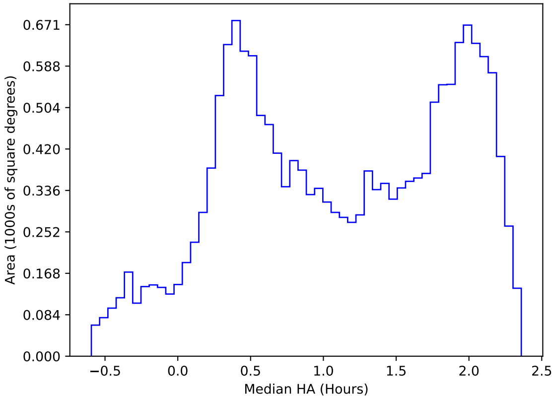
ddf_acor_sf15_lsf30_lsr50_v3.4_10yrs WFD z band: Median HA
