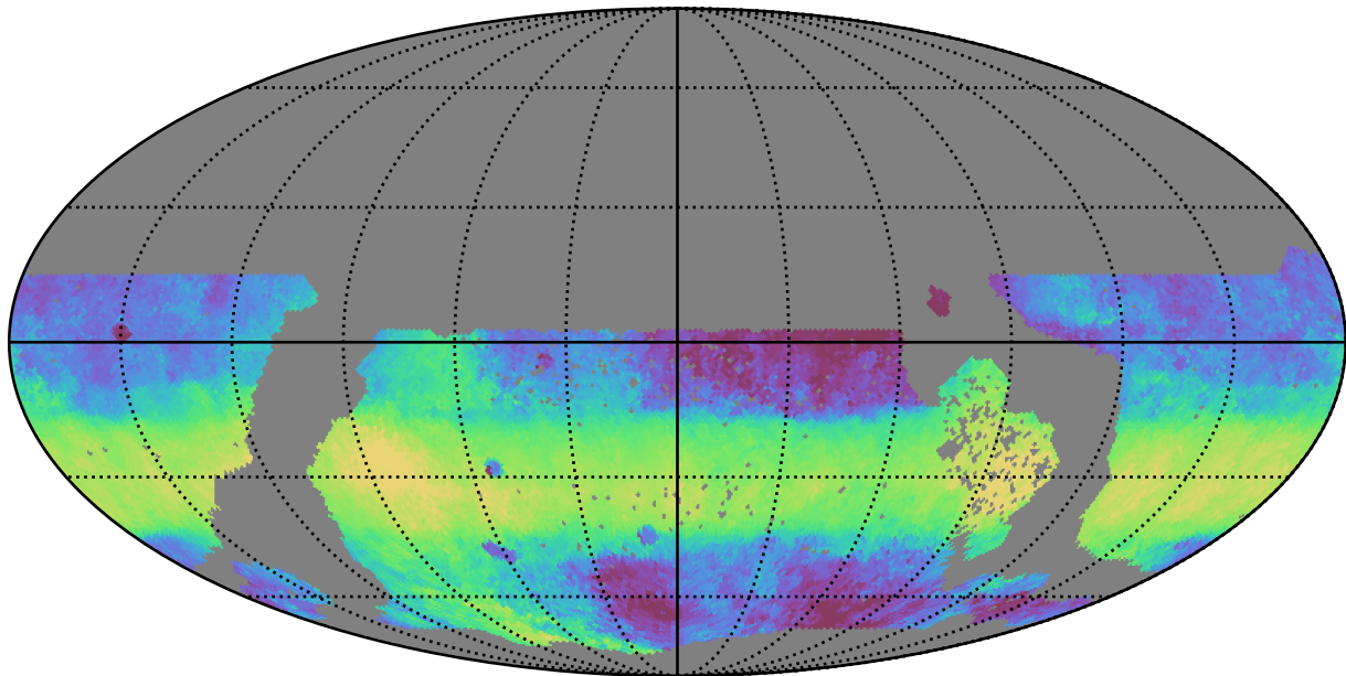
ddf_acor_sf15_lsf30_lsr50_v3.4_10yrs WFD y band: Median HA
