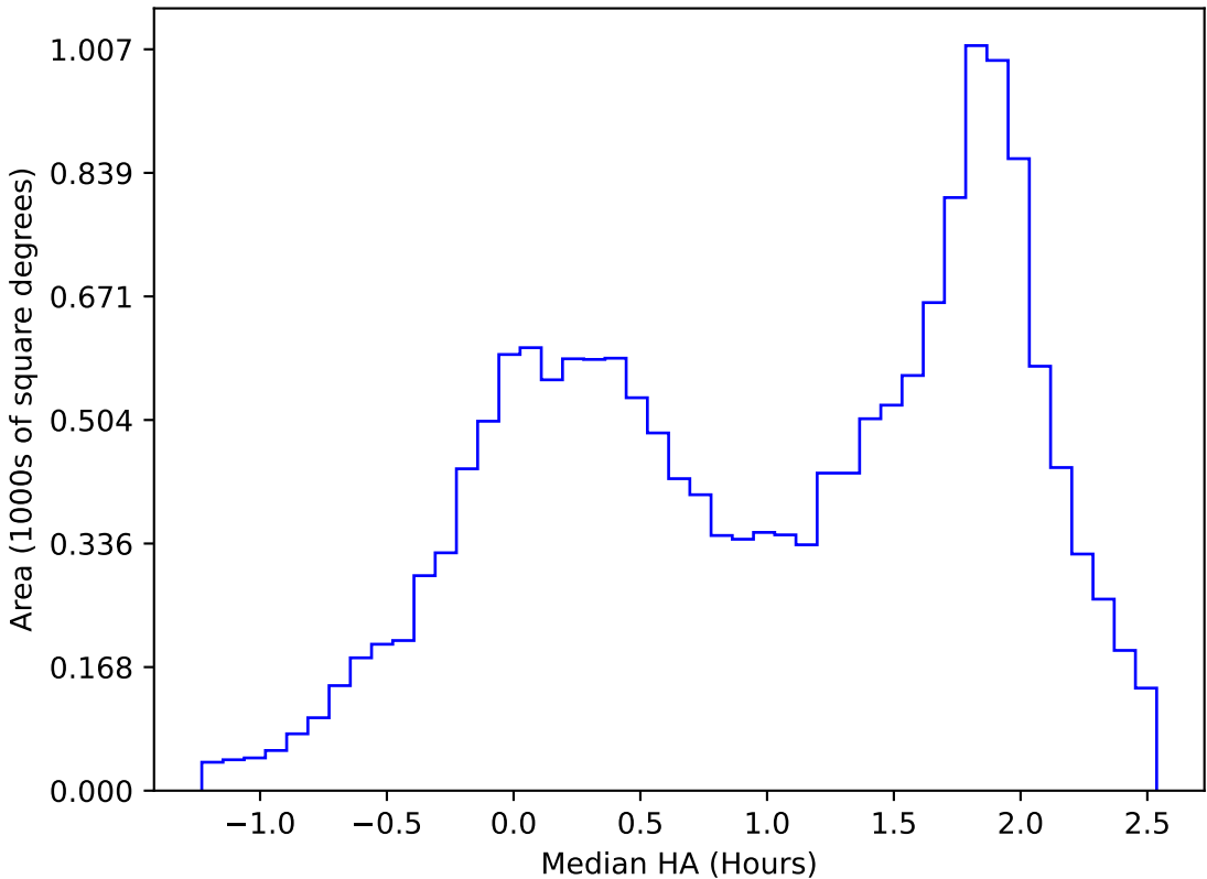
ddf_acor_sf15_lsf30_lsr50_v3.4_10yrs WFD u band: Median HA
