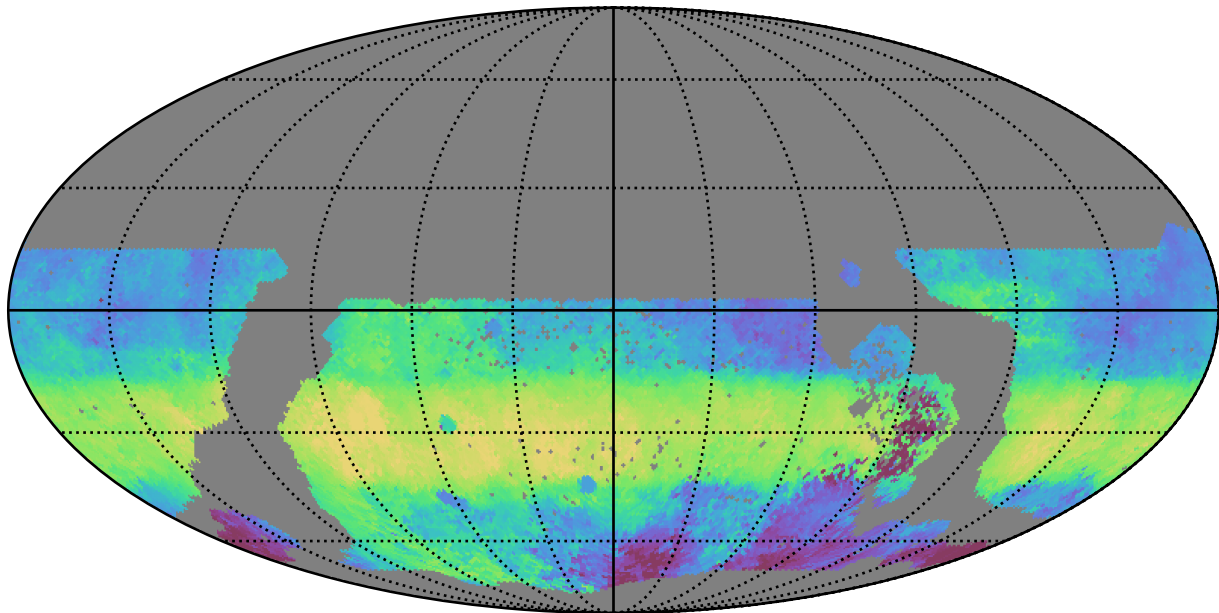
ddf_acor_sf15_lsf30_lsr50_v3.4_10yrs WFD g band: Median HA
