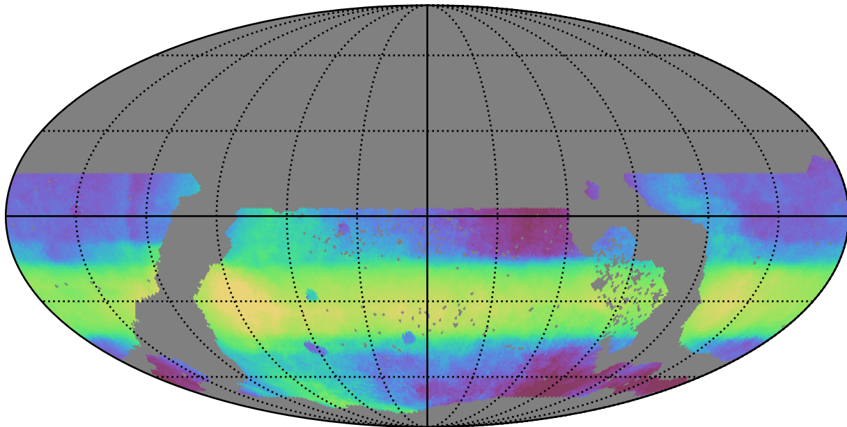
ddf_acor_sf15_lsf30_lsr50_v3.4_10yrs WFD all bands: Median HA
