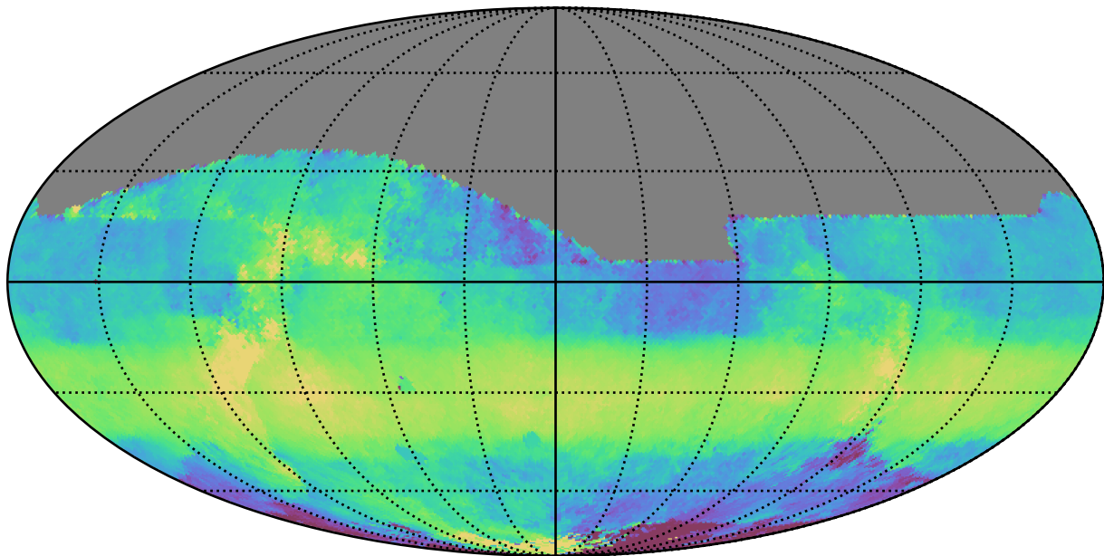
ddf_acor_sf15_lsf30_lsr50_v3.4_10yrs All sky z band: Median HA
