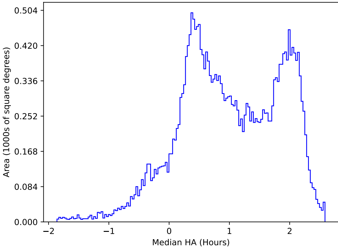
ddf_acor_sf15_ls30_lsr50_v3.4_10yrs All sky z band: Median HA
