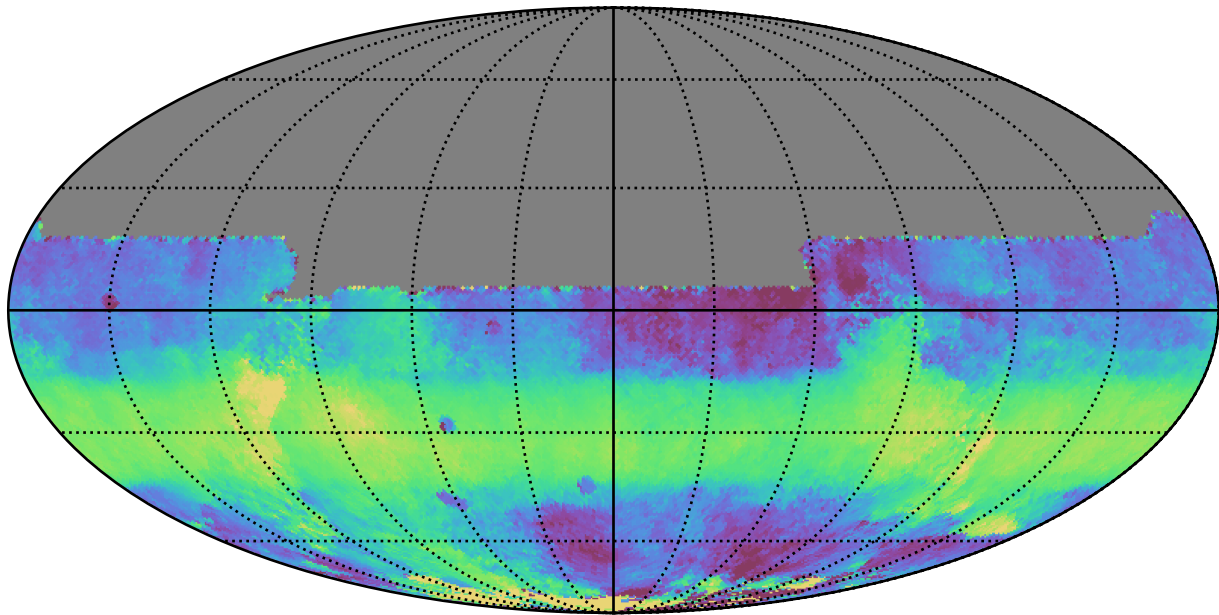
ddf_acor_sf15_lsf30_lsr50_v3.4_10yrs All sky y band: Median HA
