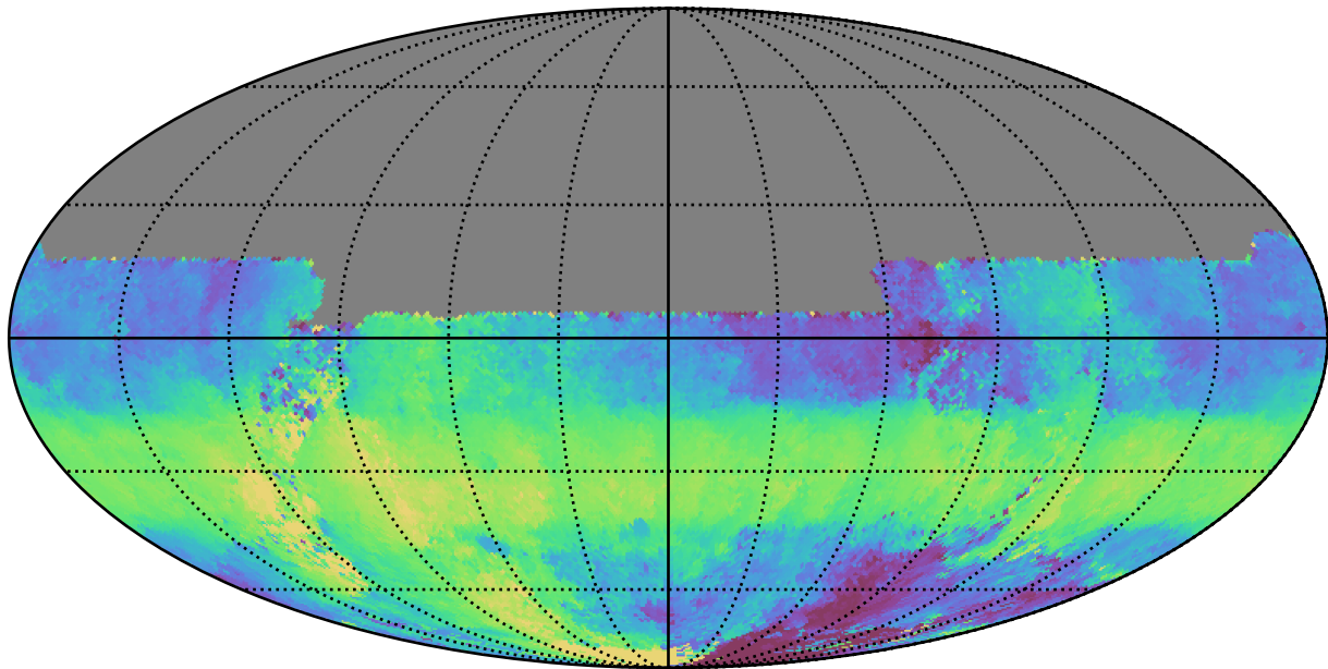
ddf_acor_sf15_lsf30_lsr50_v3.4_10yrs All sky u band: Median HA
