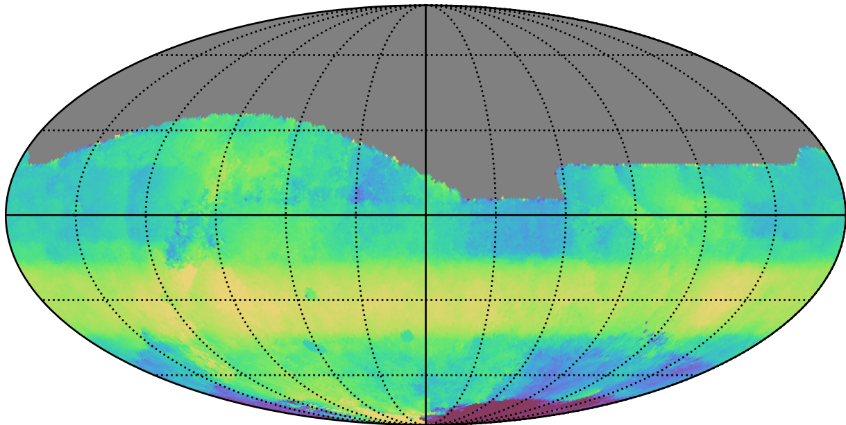
ddf_acor_sf15_lsf30_lsr50_v3.4_10yrs All sky r band: Median HA
